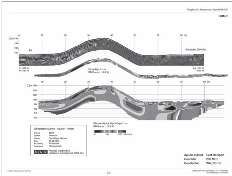
Fig. 10. Georadar and geoelectric profiles of the hill-fort's main rampart (by C. Klein).
