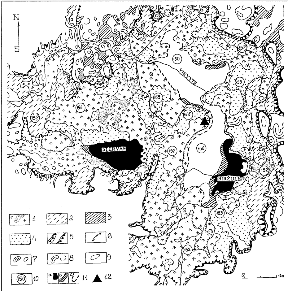
Fig. 2. Geomorphological scheme of Biržulis area (compiled by R. Guobytė 1996). 1. The bottom of the depression, with sand and peat. 2. The fragments sediments? areas? of abrasion relief in Varniai depression. 3. Boggy inter-hill depressions, with peat in the bottom. 4. The fragments sediments? areas? of accumulative relief in Varniai depression. 5. Slopes of ice contact and abrasion origin. 6. Slopes of accumulative origin. 7. Moraine hills, medium and large. 8. Low elongated moraine hills. 9. Small moraine hills. 10. Altitudes above sea level for relief in the Varniai depression. 11. Outlines of the lakes: a) on the satellite orthophoto map of 1992, b) on the aerial photo of 1979, c) on the aerial photo of 1952. 12. Location of palynological investigations
